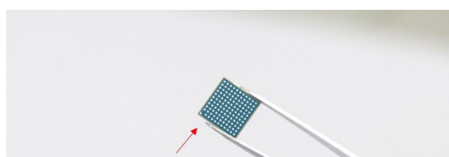
The entire all-digital PLL fits in a 50 \times 72 \mu\text{m}^2 region, making it the smallest PLL to date.
