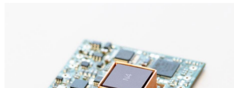
Figure 1. Prototype of the atomic clock (33mm x 38mm x 9mm): A newly developed compact ULPACs, mounted on small satellites, automobiles, and smartphones, accelerate the realization of seamless and on-demand mobile communication networks.
