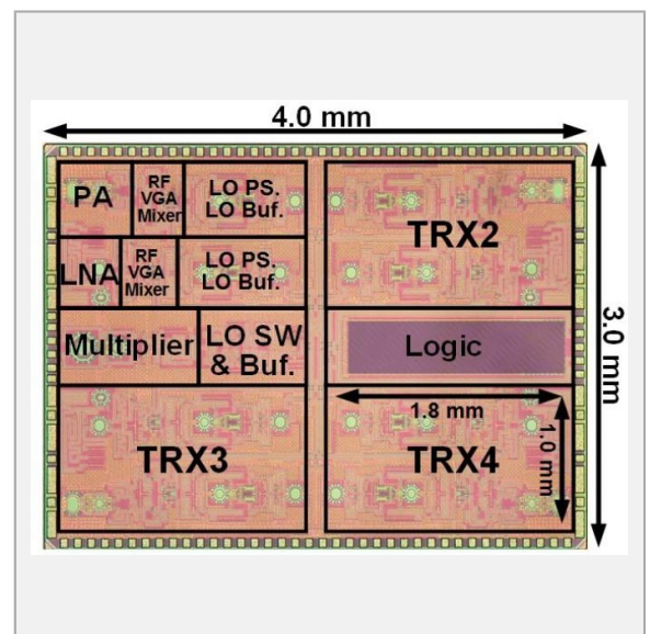
IMAGE: THE FABRICATED TRANSCEIVER ONLY MEASURES 3 MM × 4 MM AND CONSISTS OF FOUR TRANSMITTING AND RECEIVING ELEMENTS. THE SUBCOMPONENTS OF TRX1 ARE DISPLAYED. view more
